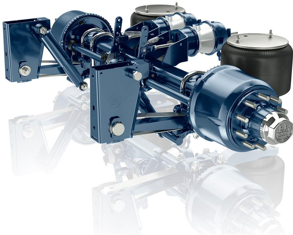
12-tonne Airlight II suspension unit for low loaders.
